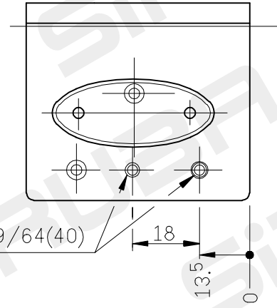
TG12F HOLE DIAGRAM
